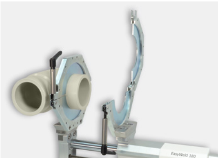
Narrow master clamps The optional narrow master clamps for the machine chassis allow easy and user-friendly clamping of even the shortest pipes and fittings.
