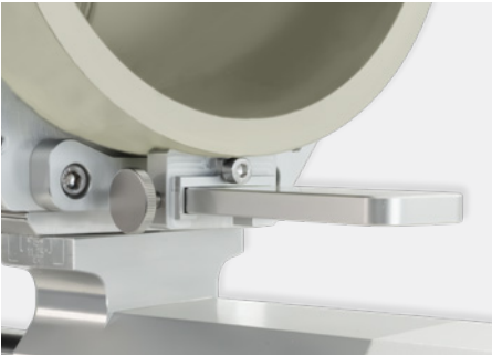
Pipe rest The pipe rest moves with the swivelling and adjustment of the clamp and thus reliably supports the exact alignment of the workpiece. If space is limited, both pipe rests can be easily removed.
